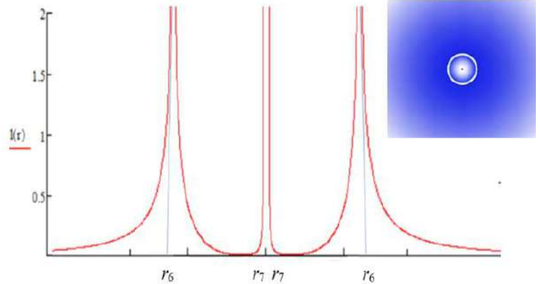
Fig. 4: Combined graphs of functions (29) and (38) of the relative elongation l_r^{(+)} of the outer side of the \lambda_{-12,-15} -vacuum (i.e., the subcont) outside and inside the core of the "electron"
