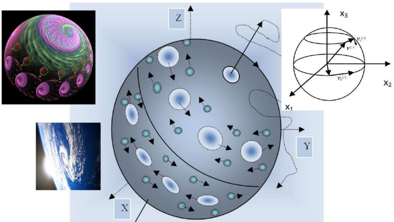
Fig. 13: Cyclones and anticyclones on the surface of the rotating core of a vacuum formation (in particular, an "electron") are similar to the circulation of air on the surface of a planet
