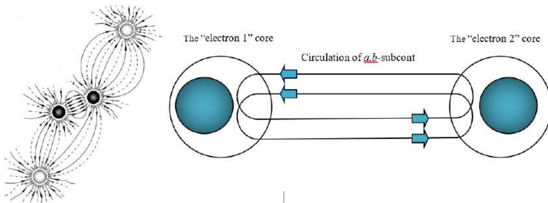
Fig. 20: Schematic representation of the average circulation of the a -subcont and b -subcont between the raqiyas of the "electron 1" and "electron 2"
