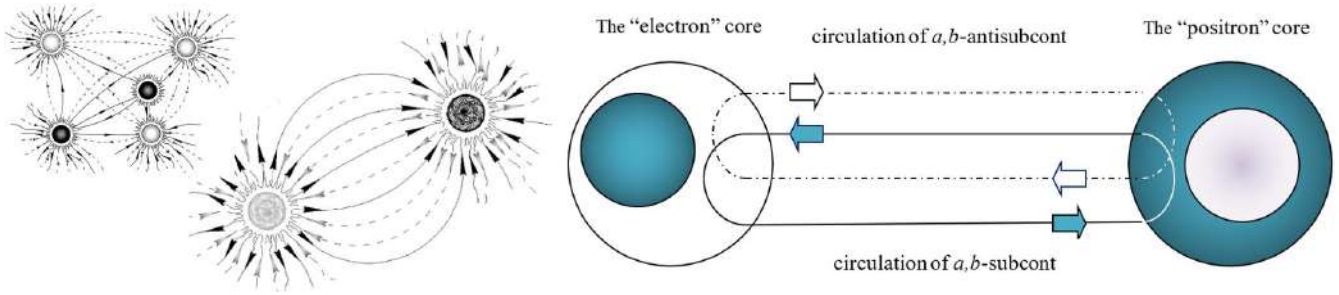
Fig. 18: Schematic representation of the average circulation of a,b -subcont and a,b -antisubcont between the "electron" and "positron" raqiyas
