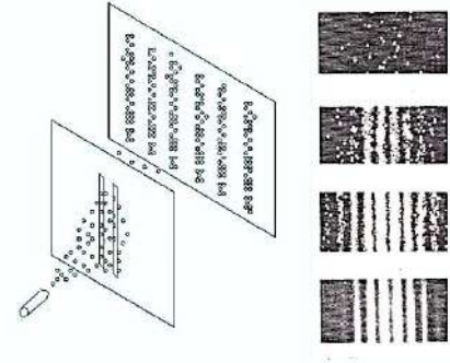
Fig. 17: Electron diffraction on two slits
