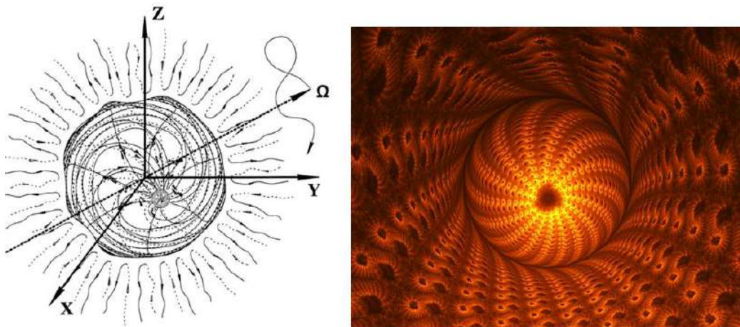
Fig. 12: The rotation of the "electron" core has two components: 1) rotation around the instantaneous axis, and 2) chaotic change in the direction of the rotation axis itself
